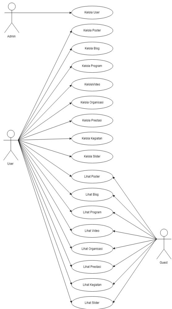
Gambar 4.1. Use Case sistem media online M-DOCS.
