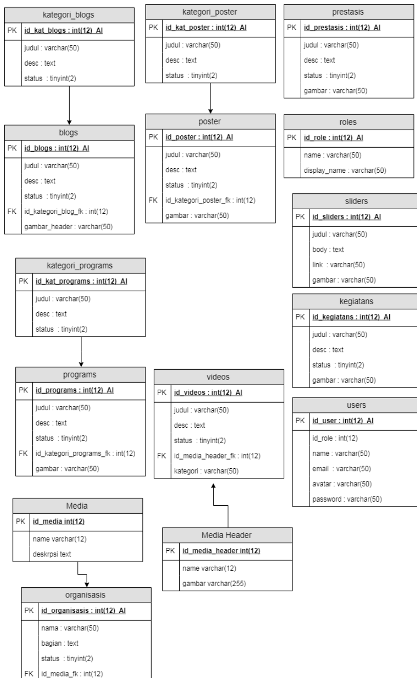
Gambar 4.2. Class Diagram sistem media online M-DOCS.
