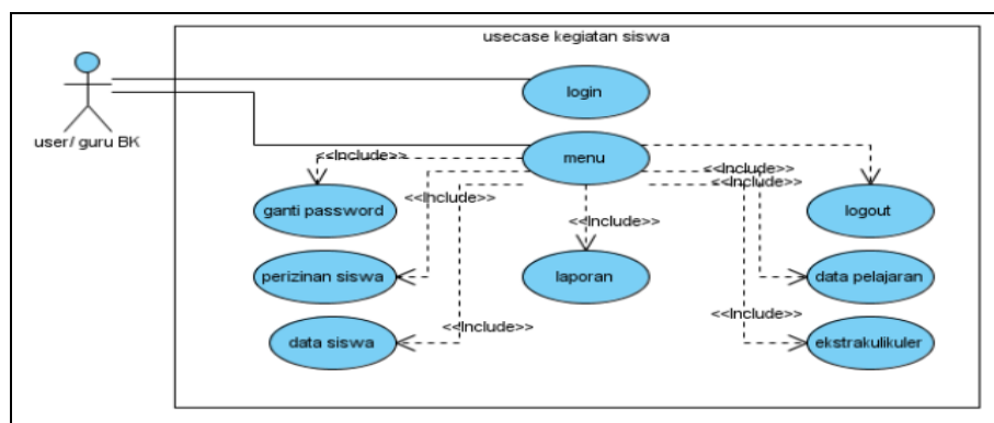
Gambar 2 Use Case Diagram User
